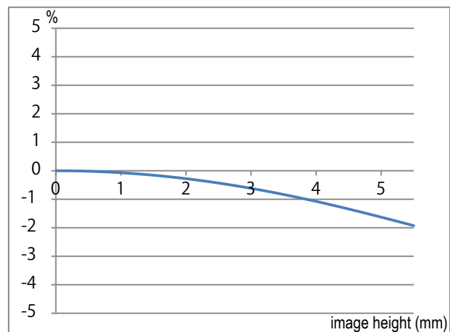
Distortion
