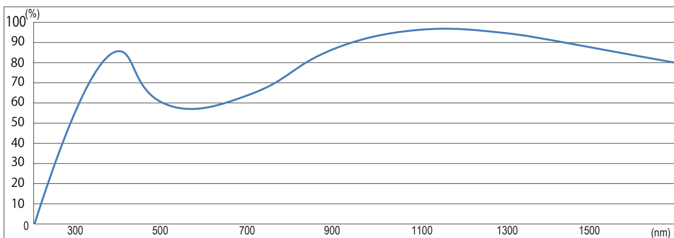
Spectral Transmittance
